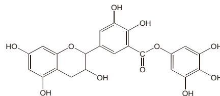
▲ (-)-Epigallocatechingallate (EGCg)
